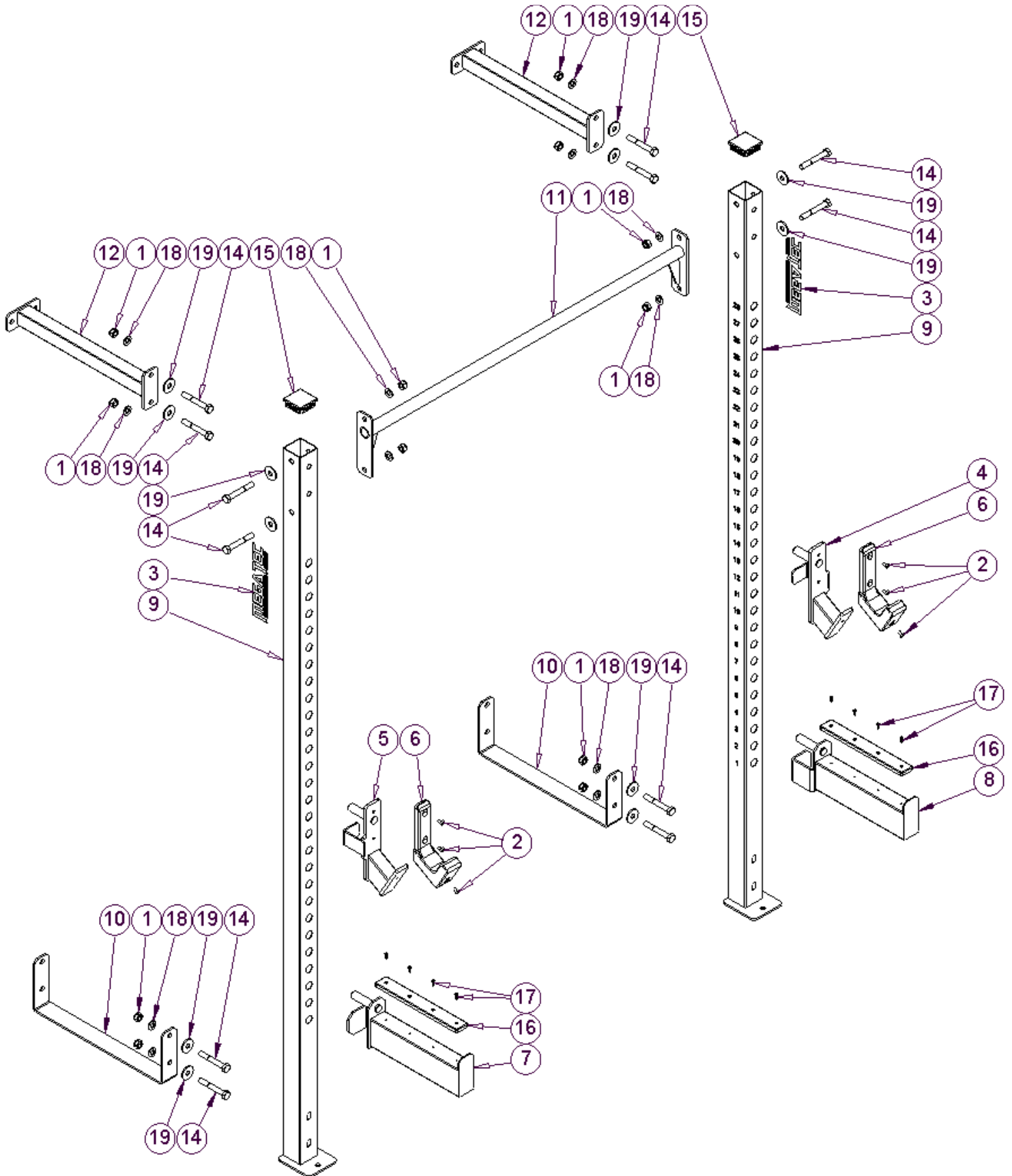
MT-HR-WM-10 HALF RACK WALL
