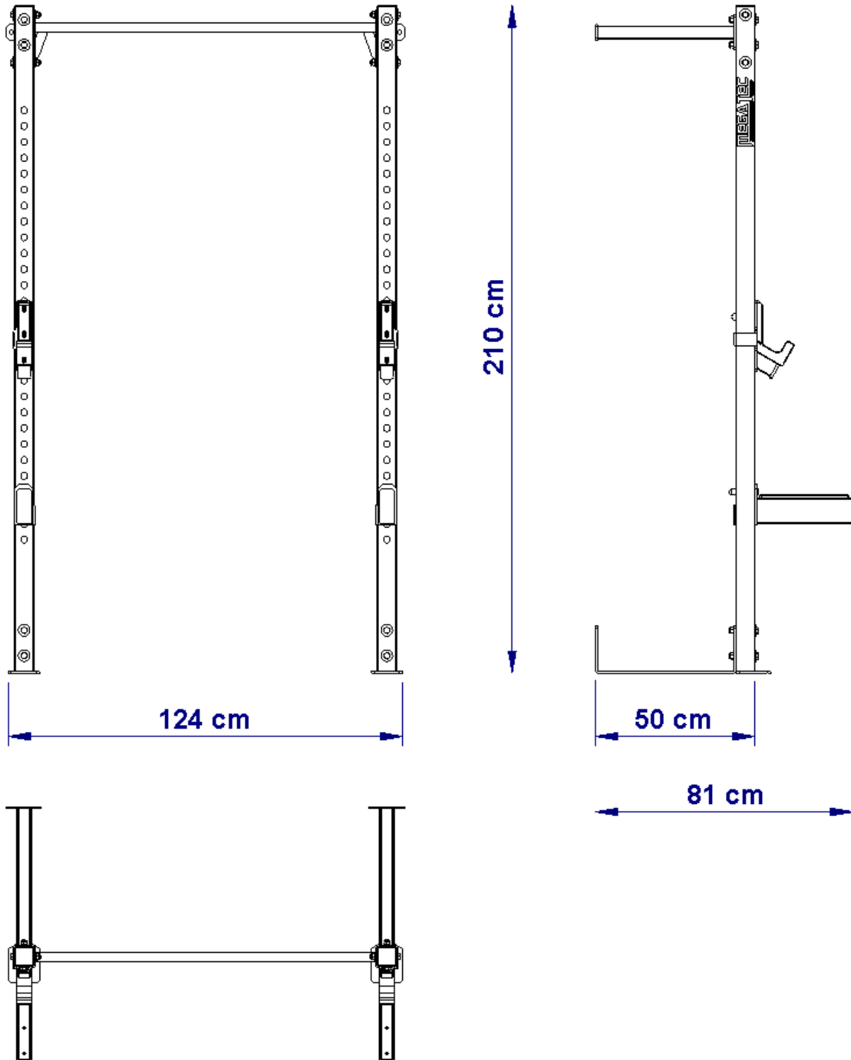
MT-HR-WM-10 HALF RACK WALL
